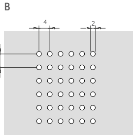
For width: 100 - 150 - 200 Perforation area: regular Inter-axes: 4x7 mm Perforation surface: 11% approx.
